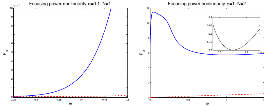
FIGURE 9. Numerical power for the focusing DNLS with power nonlinearity and (a) \sigma = 0.1, N = 1, \epsilon = 1 ( \sigma < \frac{2}{N} -no excitation threshold), (b) \sigma = 1, N = 2, \epsilon = 1 ( \sigma = \frac{2}{N} -excitation threshold). The inset in (b) shows a magnification of the region where the power reaches its minimum value. Dashed line corresponds to lower bound (137)
