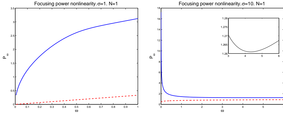
FIGURE 8. Numerical power for the focusing DNLS with power nonlinearity and (a) \sigma = 1, N = 1, \epsilon = 1 ( \sigma < \frac{2}{N} -no excitation threshold), (b) \sigma = 10, N = 1, \epsilon = 1 ( \sigma > \frac{2}{N} -excitation threshold). The inset in (b) shows a magnification of the region where the power reaches its minimum value. Dashed line corresponds to lower bound (137)
