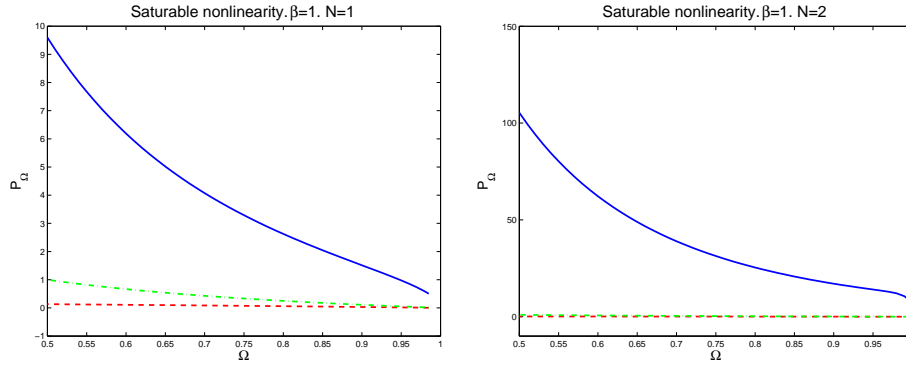
FIGURE 2. Dependence of the power with respect to the frequency for 1D and 2D lattices of the focusing DNLS with saturable nonlinearity for \beta = 1 and \epsilon = 1 . Power decreases approaching the theoretical lower bounds when \Omega tends to \beta .
