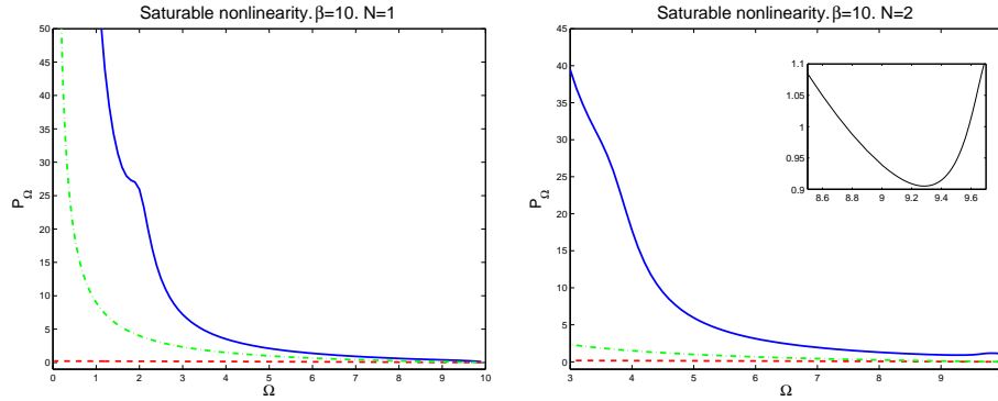
FIGURE 3. Dependence of the power with respect to the frequency for 1D and 2D lattices of the focusing DNLS with saturable nonlinearity for \beta = 10 and \epsilon = 1 . Power decreases approaching the lower bounds when \Omega tends to \beta . Increased accuracy of the variational lower bound (74), for N = 1 . An excitation threshold appears in the 2D-lattice.
