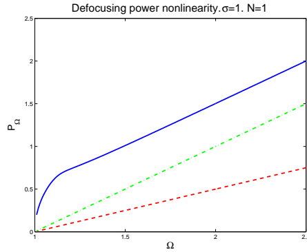
FIGURE 7. Numerical power for the defocusing DNLS with power nonlinearity case \sigma = 1 , N = 1 , \epsilon = 0.25 . The lower bounds (116) and (129), dot-dashed and dashed lines respectively, are fulfilled as threshold values.
