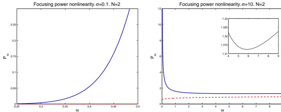
FIGURE 10. Numerical power for the focusing DNLS with power nonlinearity and (a) \sigma = 0.1 , N = 2 , \epsilon = 1 ( \sigma < \frac{2}{N} -no excitation threshold), (b) \sigma = 10 , N = 2 , \epsilon = 1 ( \sigma > \frac{2}{N} -excitation threshold). The inset in (b) shows a magnification of the region where the power reaches its minimum value. Dashed line corresponds to lower bound (137)
