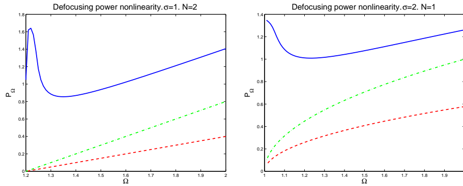
FIGURE 4. Numerical power for the defocusing DNLS with power nonlinearity and (a) \sigma = 1 , N = 2 , \epsilon = 0.15 (b) \sigma = 2 , N = 1 , \epsilon = 0.25 . The lower bounds (116) and (129), dot-dashed and dashed lines respectively, serve as thresholds for the existence of nontrivial breather solutions.
