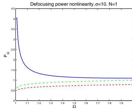
FIGURE 5. Numerical power for the defocusing DNLS with power nonlinearity and \sigma = 10 , N = 1 , \epsilon = 0.25 . Both lower bounds (116) and (129), dot-dashed and dashed lines respectively, are fulfilled as threshold values.
