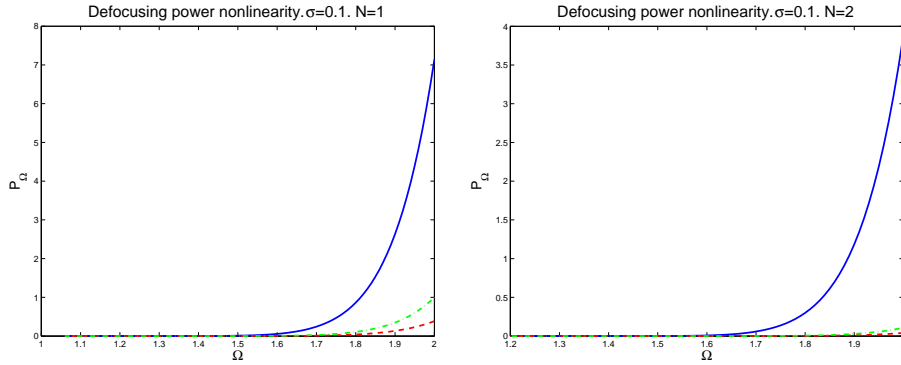
FIGURE 6. Numerical power for the defocusing DNLS with power nonlinearity case for (a) \sigma = 0.1 , N = 1 , \epsilon = 0.25 (b) \sigma = 0.1 , N = 2 , \epsilon = 0.15 . The lower bounds (116) and (129), dot-dashed and dashed lines respectively, are fulfilled as threshold values.
